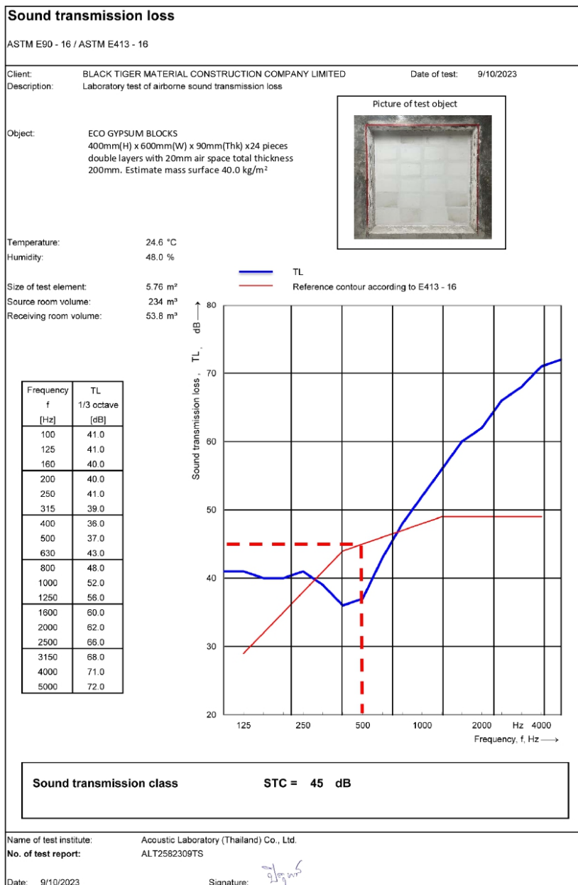
Figure 1 Rating graph of the Sound Transmission Class in accordance with the ASTM E413
